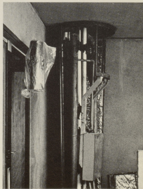
One fiberglass shaft provides mechanical and electrical services for a cluster of eight boxes.
