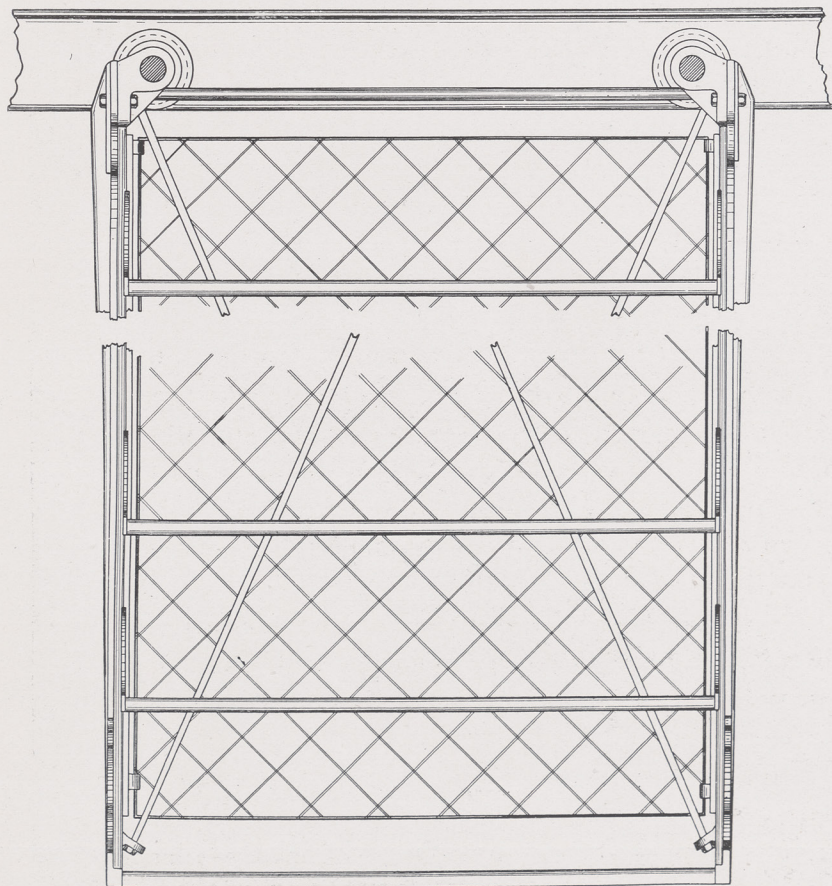
DETAILS OF ROLLING STACK.
