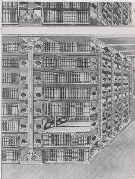
ROLLING STACK SYSTEM.
